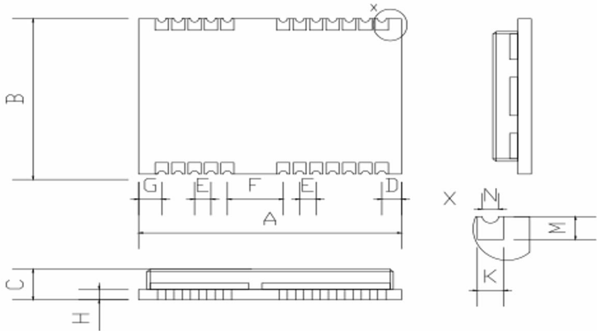
GUIDE K35 Series 24-pin LCC package mechanical drawing. All dimensions shown in millimeters.
